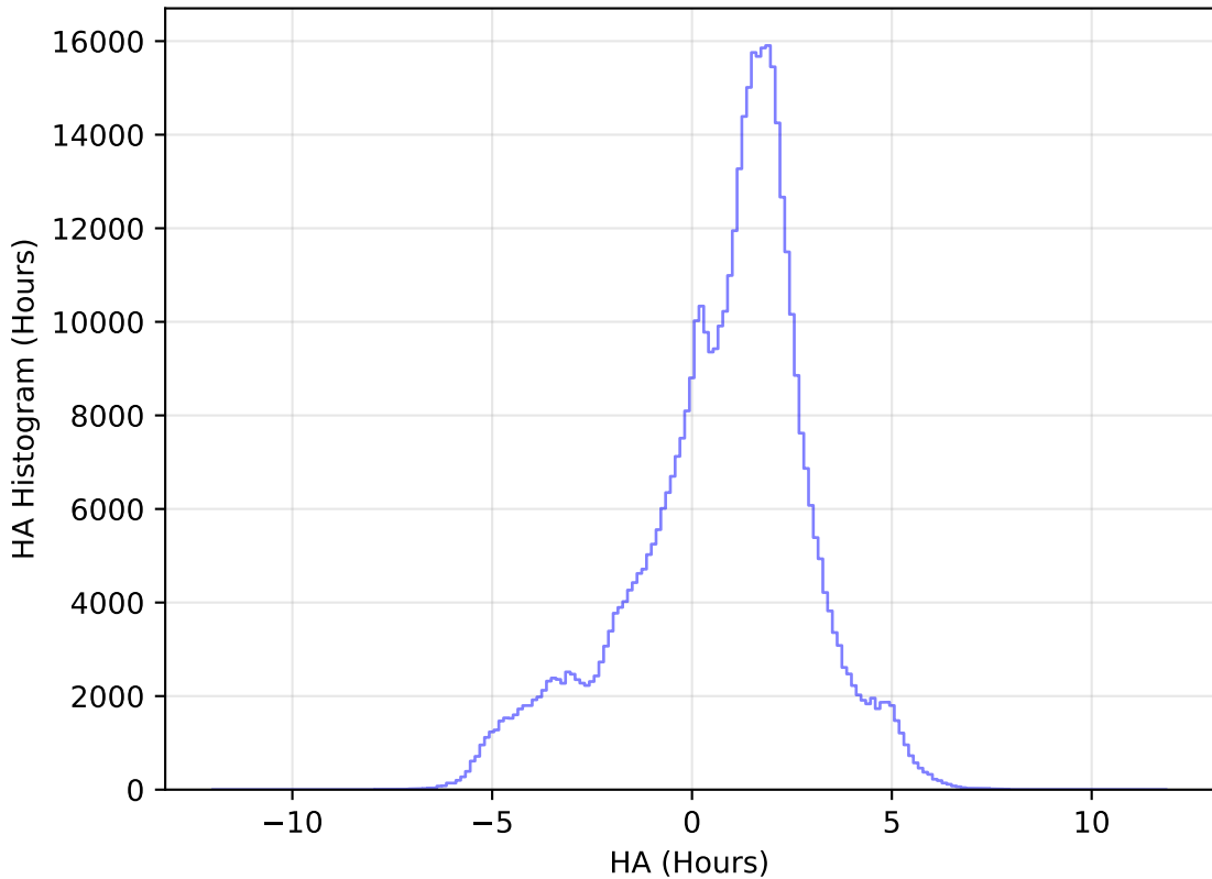
too_elab_heavy_r32_d2_gz_v3.4_10yrs All sky i band: HA Histogram
