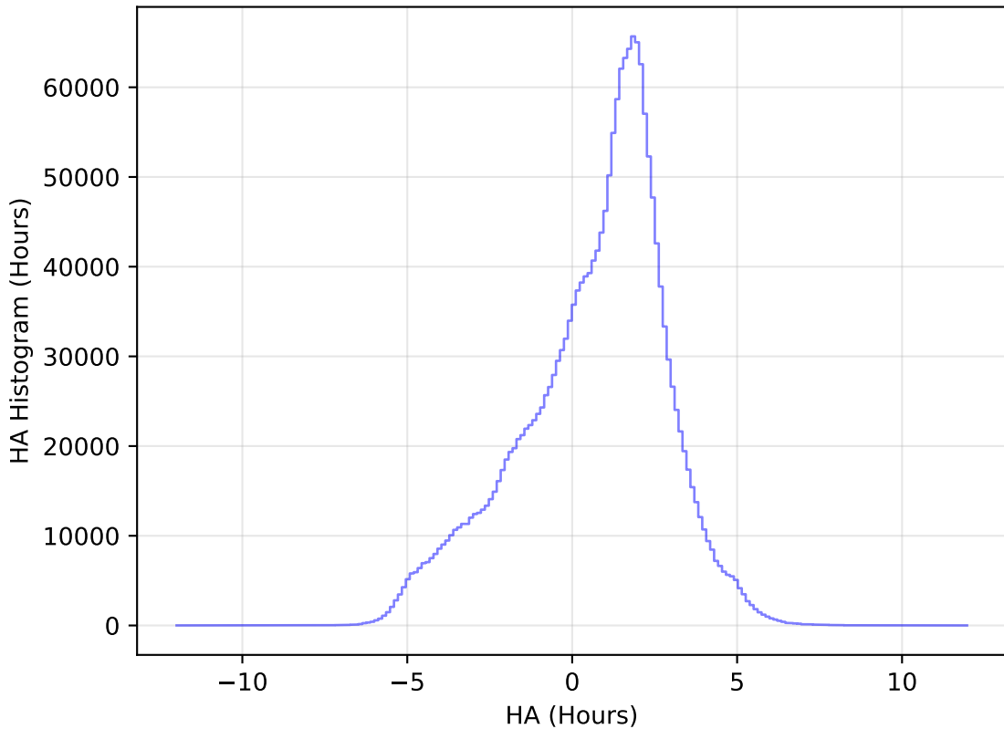
too_elab_heavy_r32_d2_gz_v3.4_10yrs All sky all bands: HA Histogram
