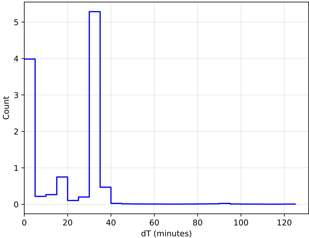
too_elab_heavy_r32_d2_gz_v3.4_10yrs WFD: DeltaT Histogram 1e6
