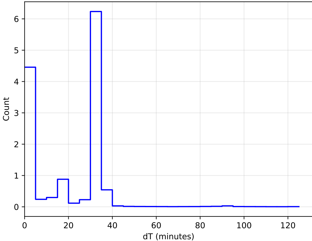
too_elab_heavy_r32_d2_gz_v3.4_10yrs All sky: DeltaT Histogram 1e6
