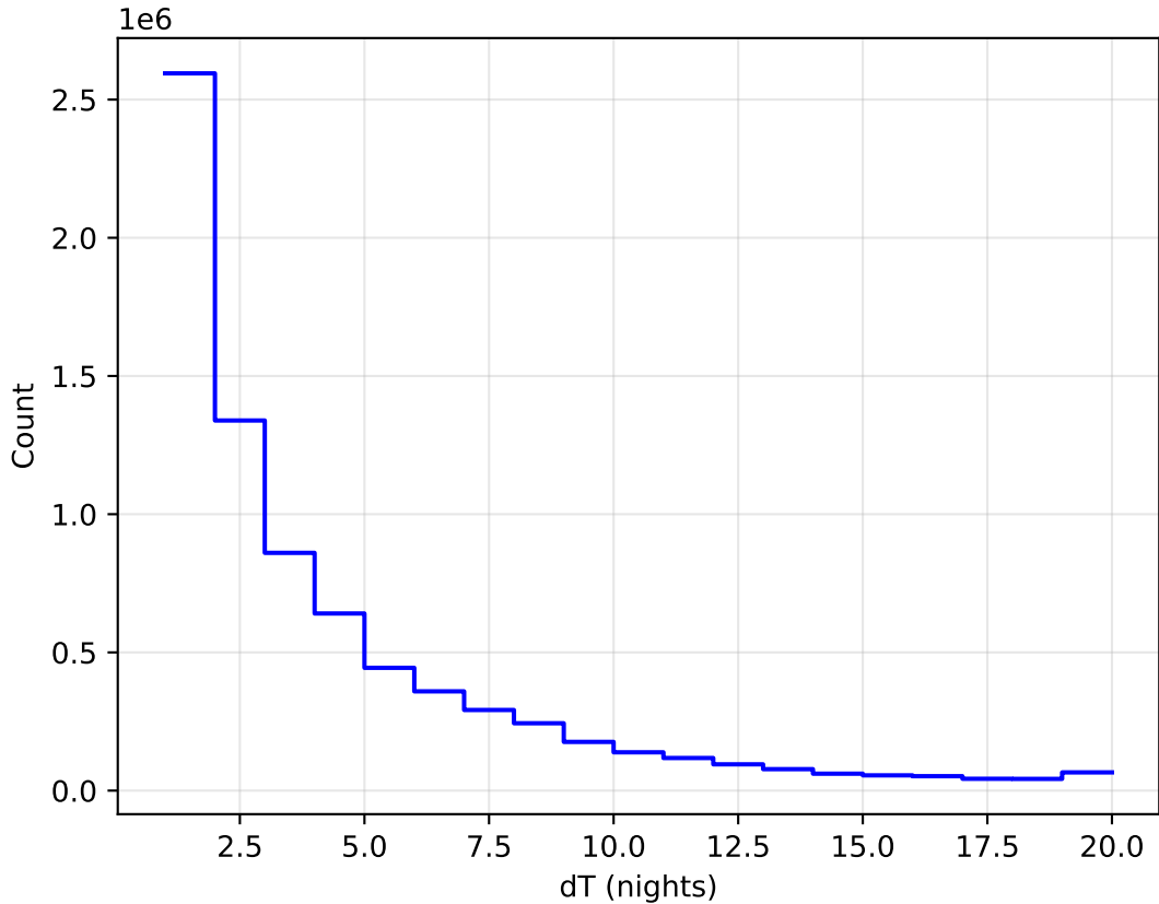
too_elab_heavy_r32_d2_gz_v3.4_10yrs WFD all bands: DeltaNight Histogram
