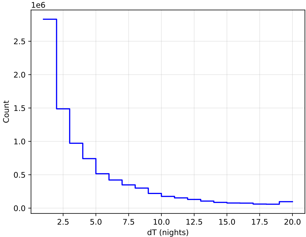
too_elab_heavy_r32_d2_gz_v3.4_10yrs All sky all bands: DeltaNight Histogram
