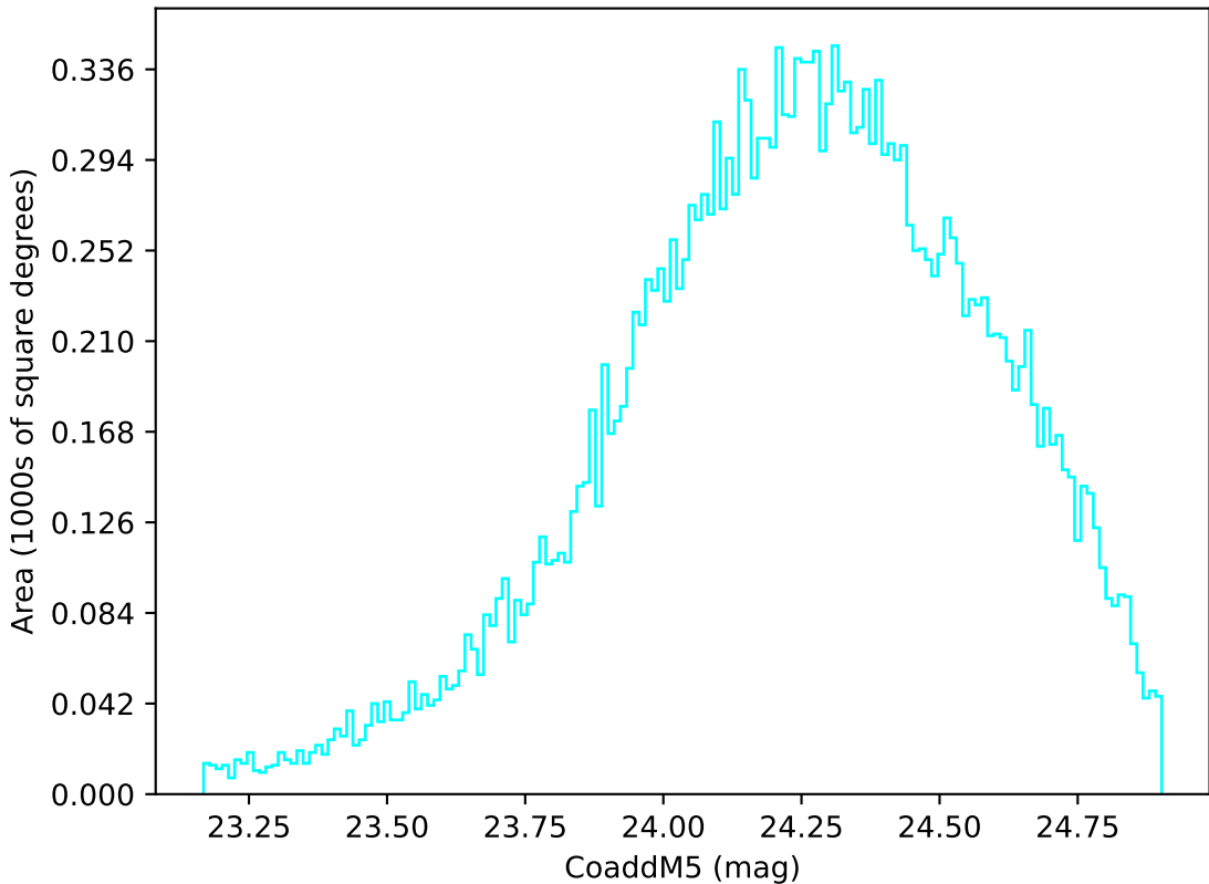
too_elab_heavy_r32_d2_gz_v3.4_10yrs Yr 1 u band: CoaddM5
