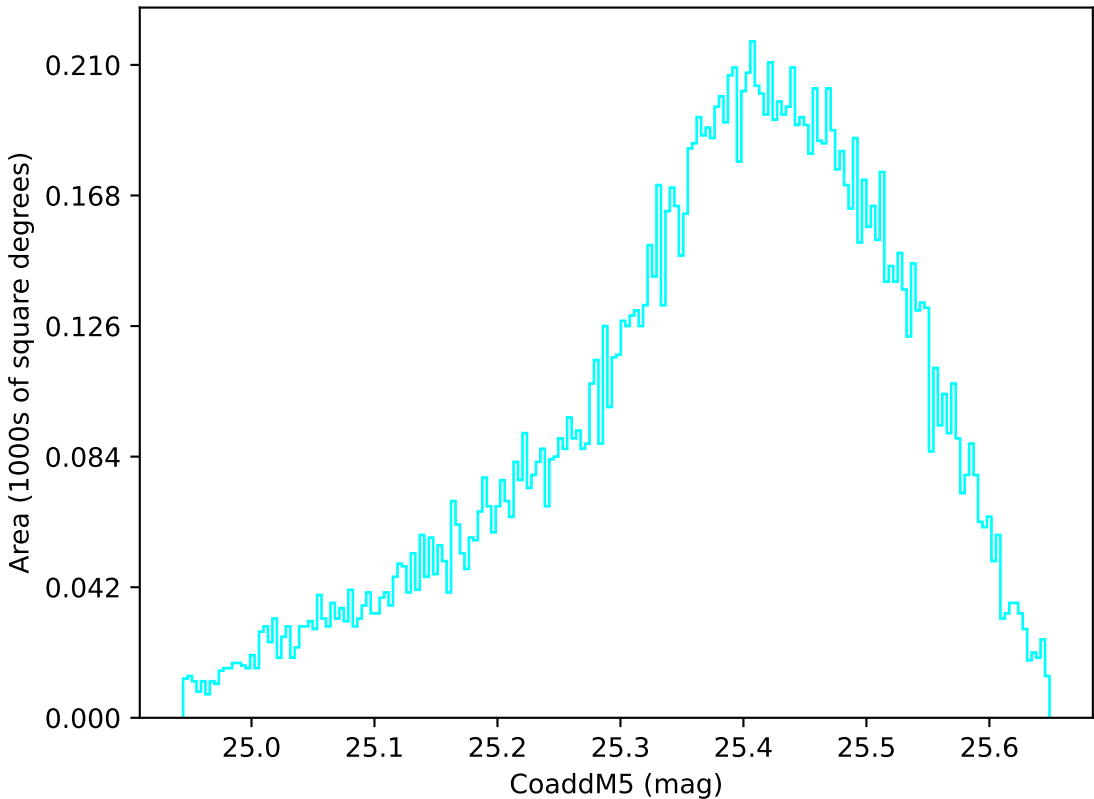
too_elab_heavy_r32_d2_gz_v3.4_10yrs WFD u band: CoaddM5
