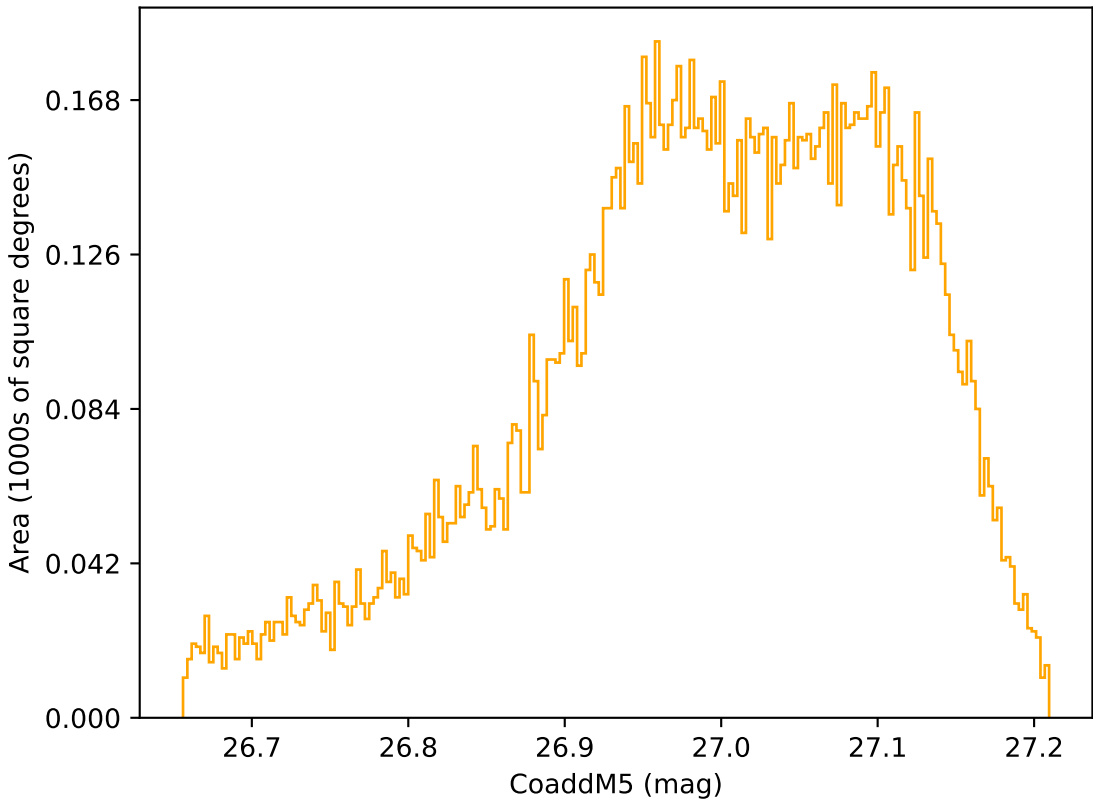
too_elab_heavy_r32_d2_gz_v3.4_10yrs WFD r band: CoaddM5
