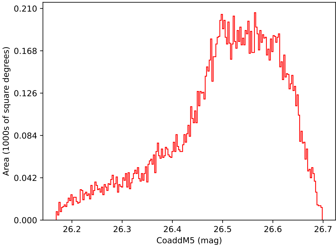
too_elab_heavy_r32_d2_gz_v3.4_10yrs WFD i band: CoaddM5
