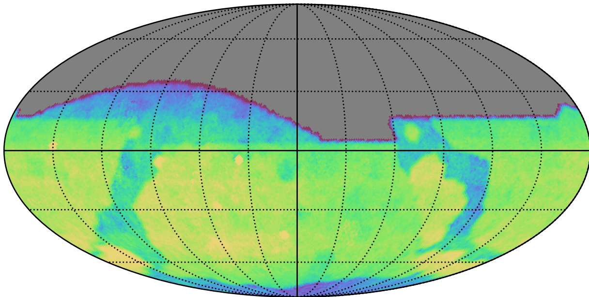
too_elab_heavy_r32_d2_gz_v3.4_10yrs All sky g band: CoaddM5
