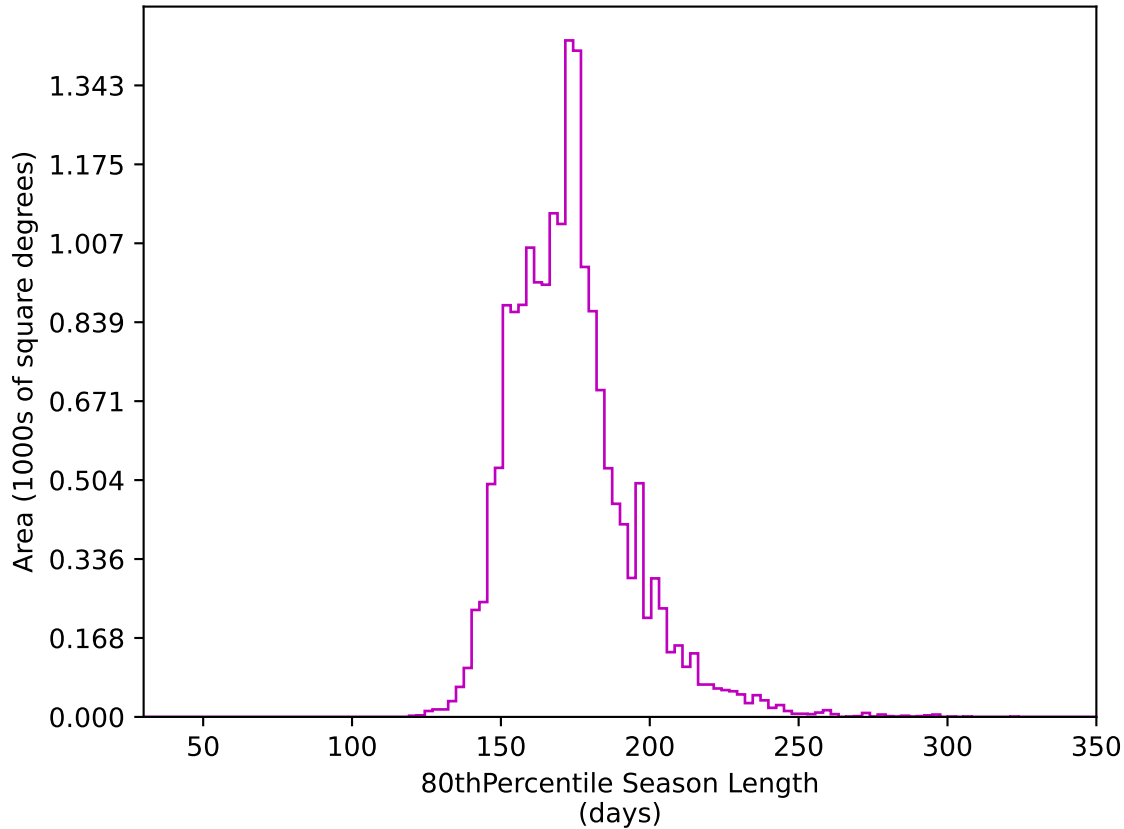
too_elab_heavy_r32_d2_gz_v3.4_10yrs WFD z band: 80thPercentile Season Length
