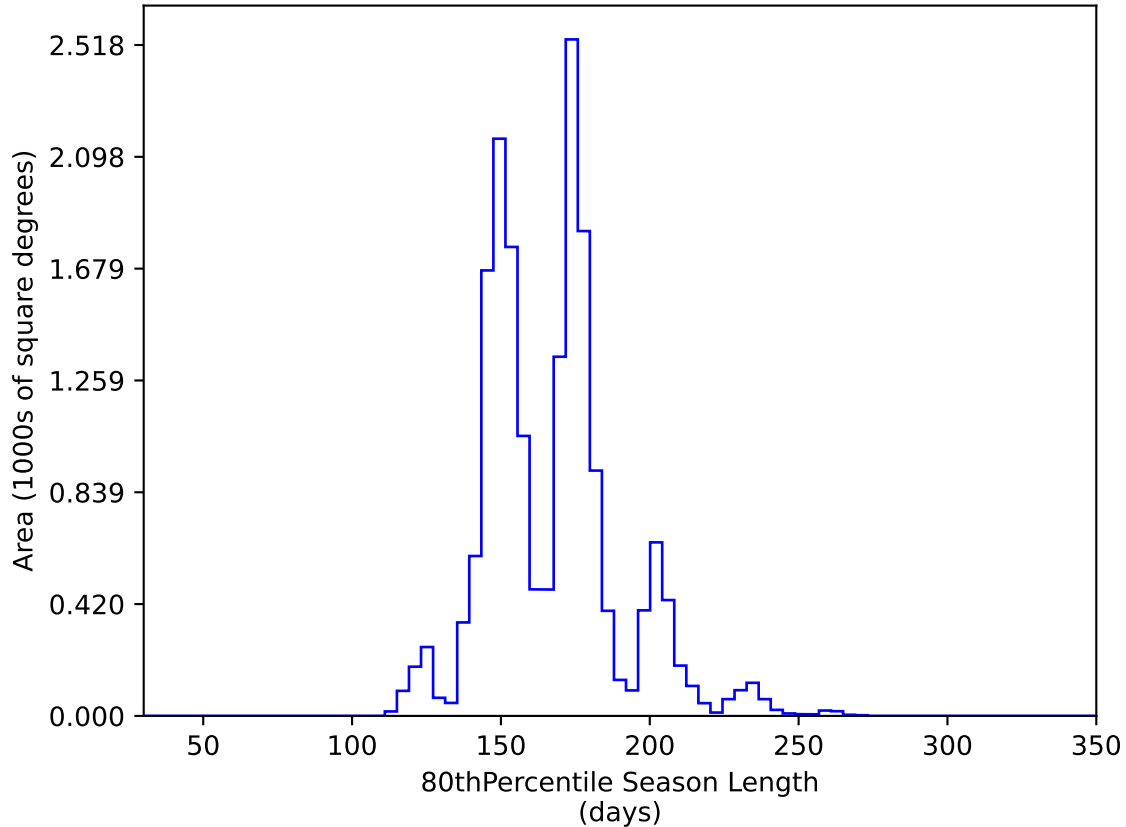
too_elab_heavy_r32_d2_gz_v3.4_10yrs WFD y band: 80thPercentile Season Length
