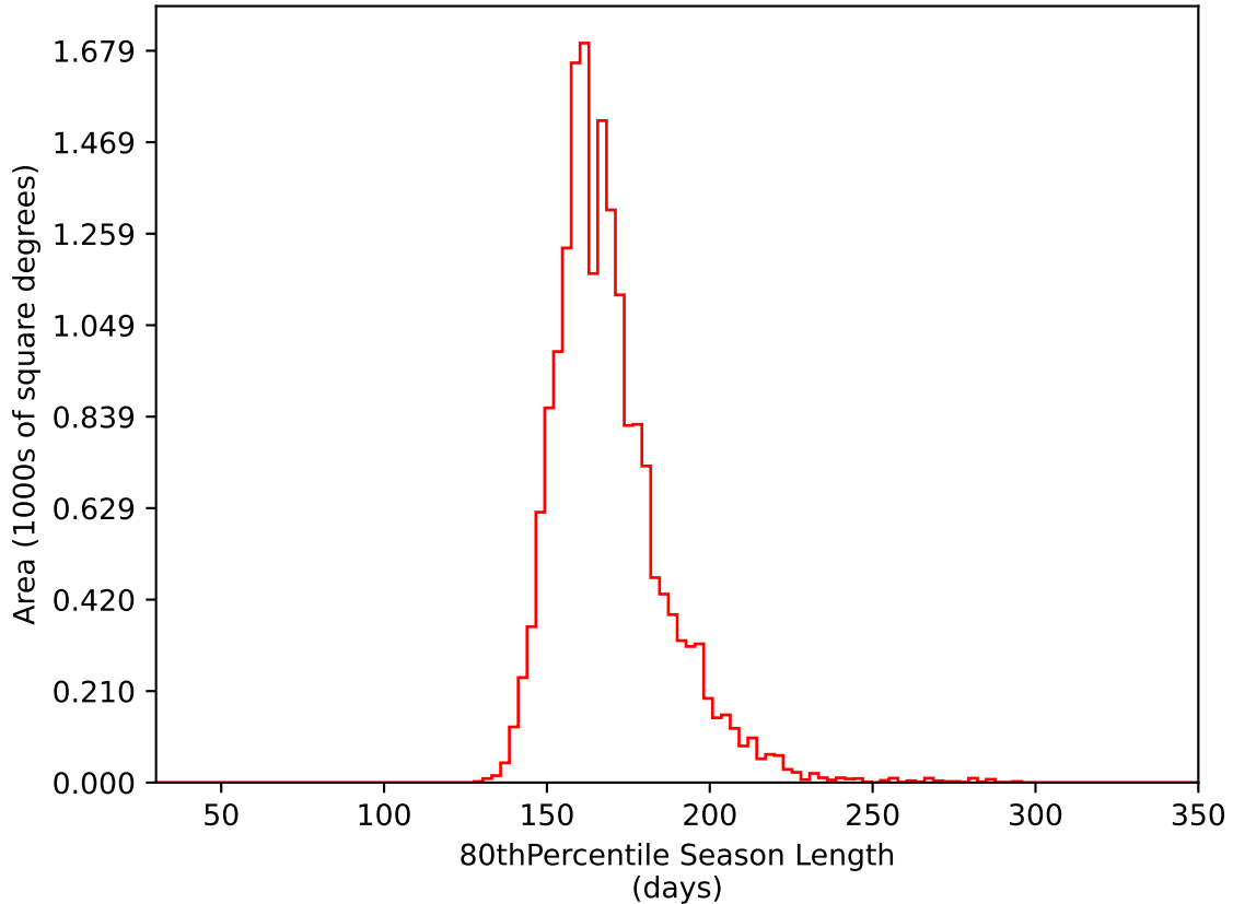
too_elab_heavy_r32_d2_gz_v3.4_10yrs WFD i band: 80thPercentile Season Length
