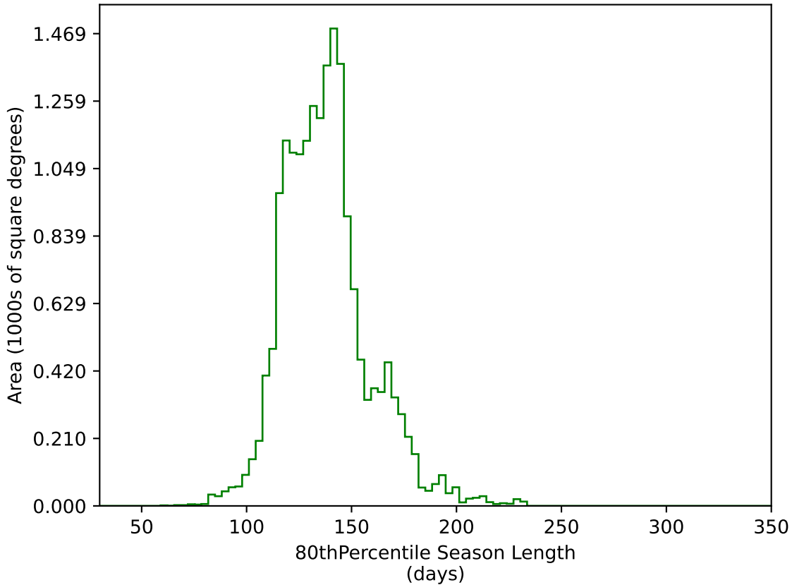
too_elab_heavy_r32_d2_gz_v3.4_10yrs WFD g band: 80thPercentile Season Length
