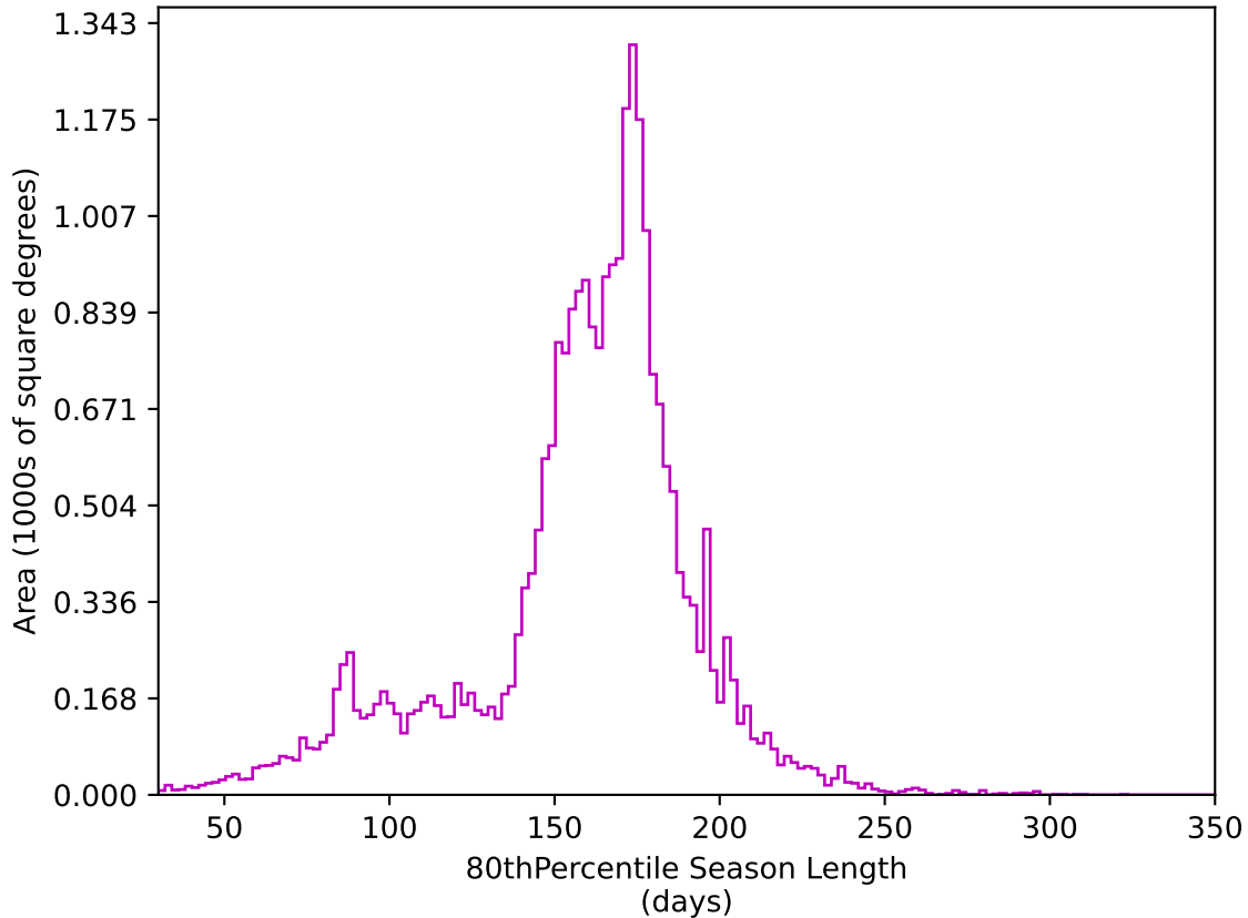
too_elab_heavy_r32_d2_gz_v3.4_10yrs All sky z band: 80thPercentile Season Length
