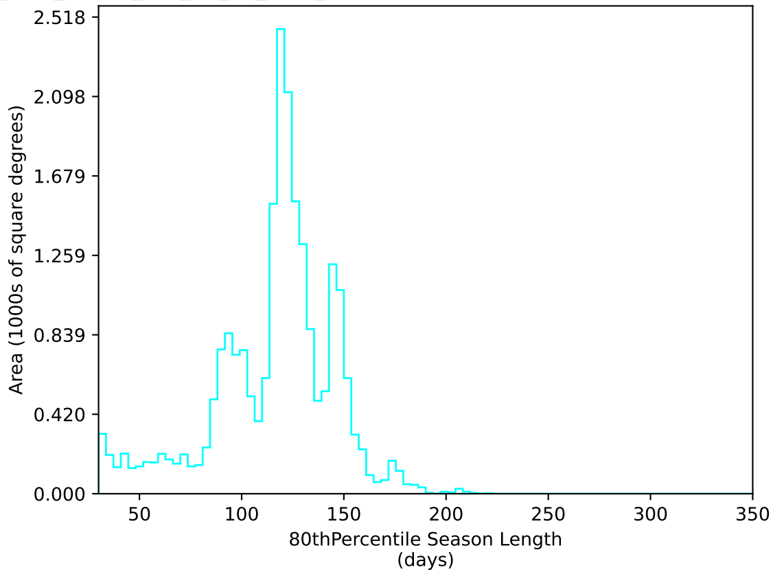
too_elab_heavy_r32_d2_gz_v3.4_10yrs All sky u band: 80thPercentile Season Length
