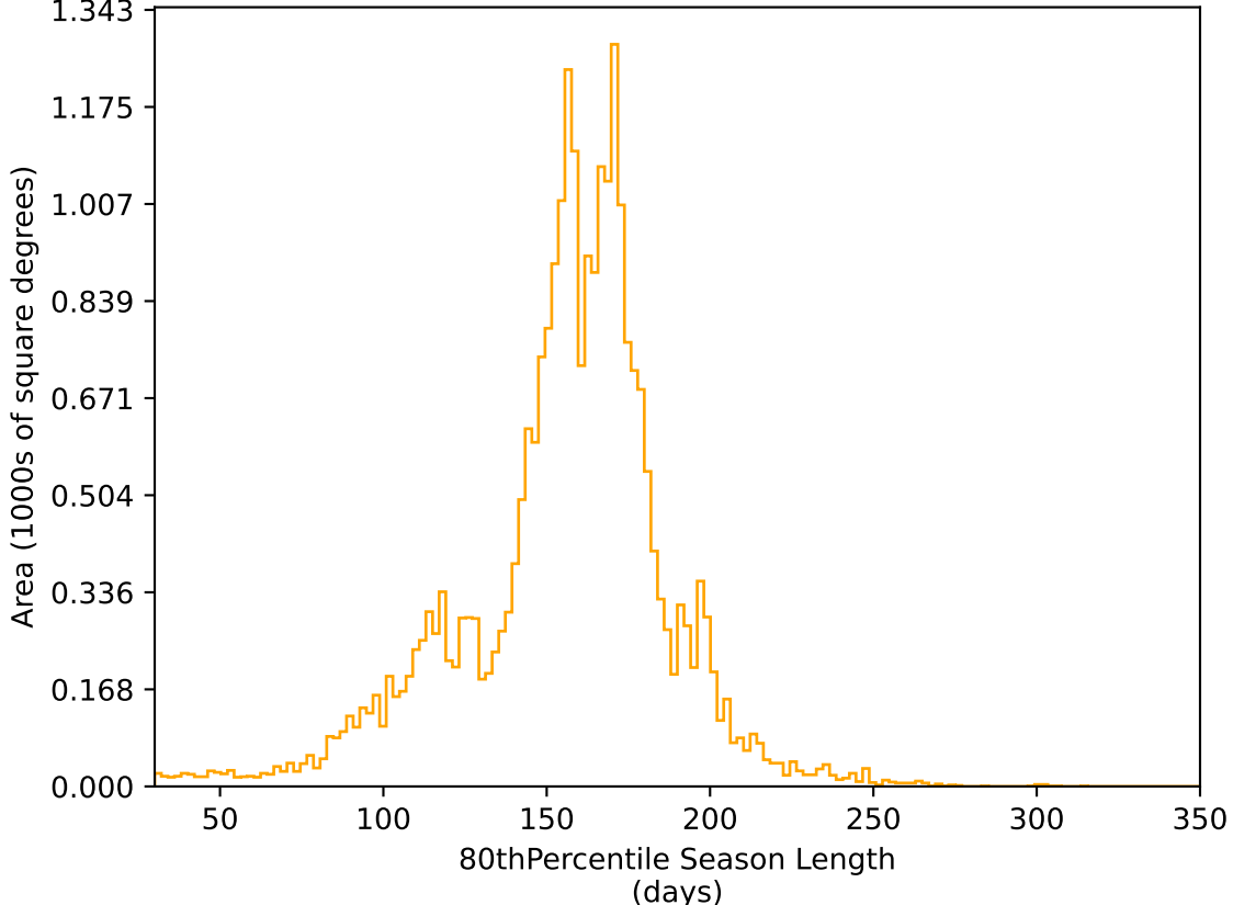
too_elab_heavy_r32_d2_gz_v3.4_10yrs All sky r band: 80thPercentile Season Length
