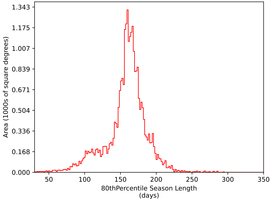
too_elab_heavy_r32_d2_gz_v3.4_10yrs All sky i band: 80thPercentile Season Length
