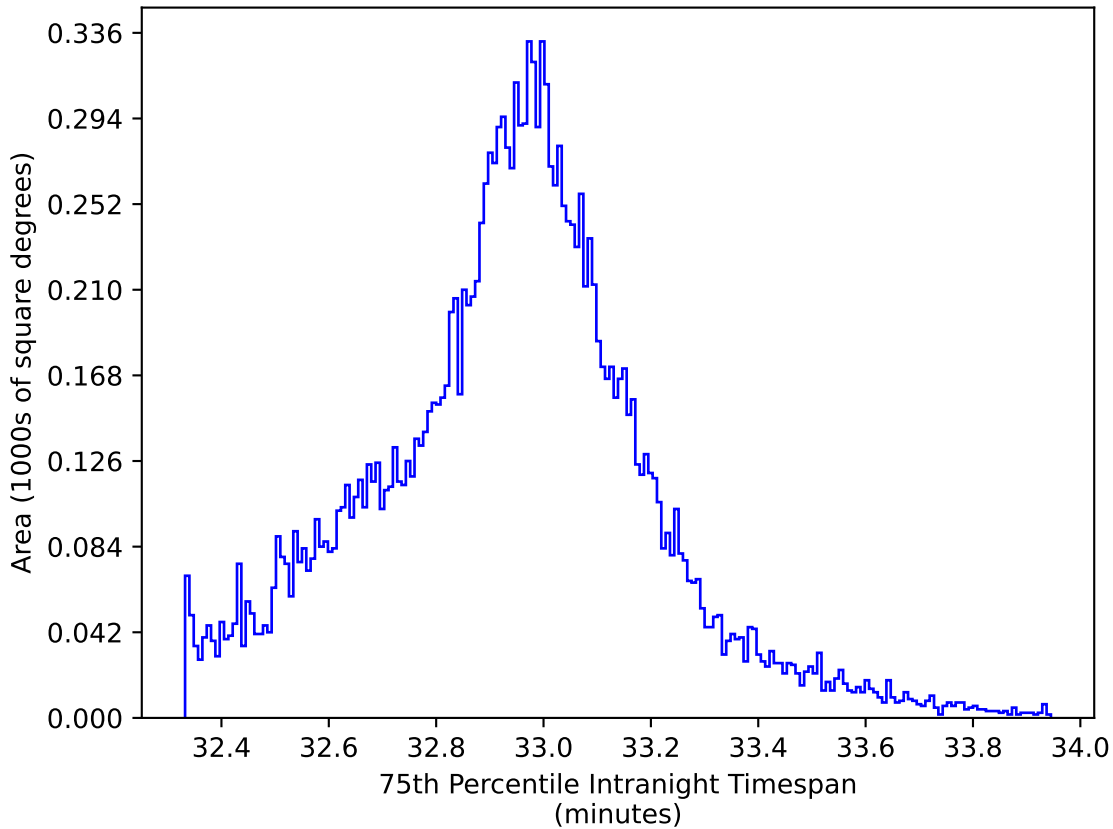
too_elab_heavy_r32_d2_gz_v3.4_10yrs WFD y band: 75th Percentile Intranight Timespan
