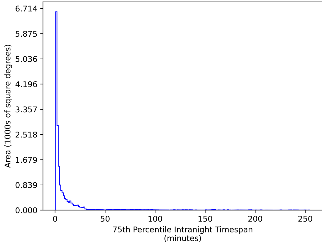
too_elab_heavy_r32_d2_gz_v3.4_10yrs WFD u band: 75th Percentile Intranight Timespan
