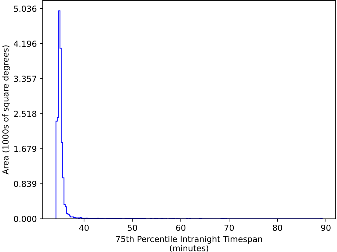
too_elab_heavy_r32_d2_gz_v3.4_10yrs WFD ri bands: 75th Percentile Intranight Timespan
