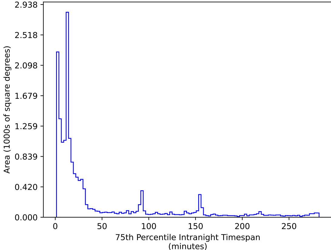
too_elab_heavy_r32_d2_gz_v3.4_10yrs WFD r band: 75th Percentile Intranight Timespan
