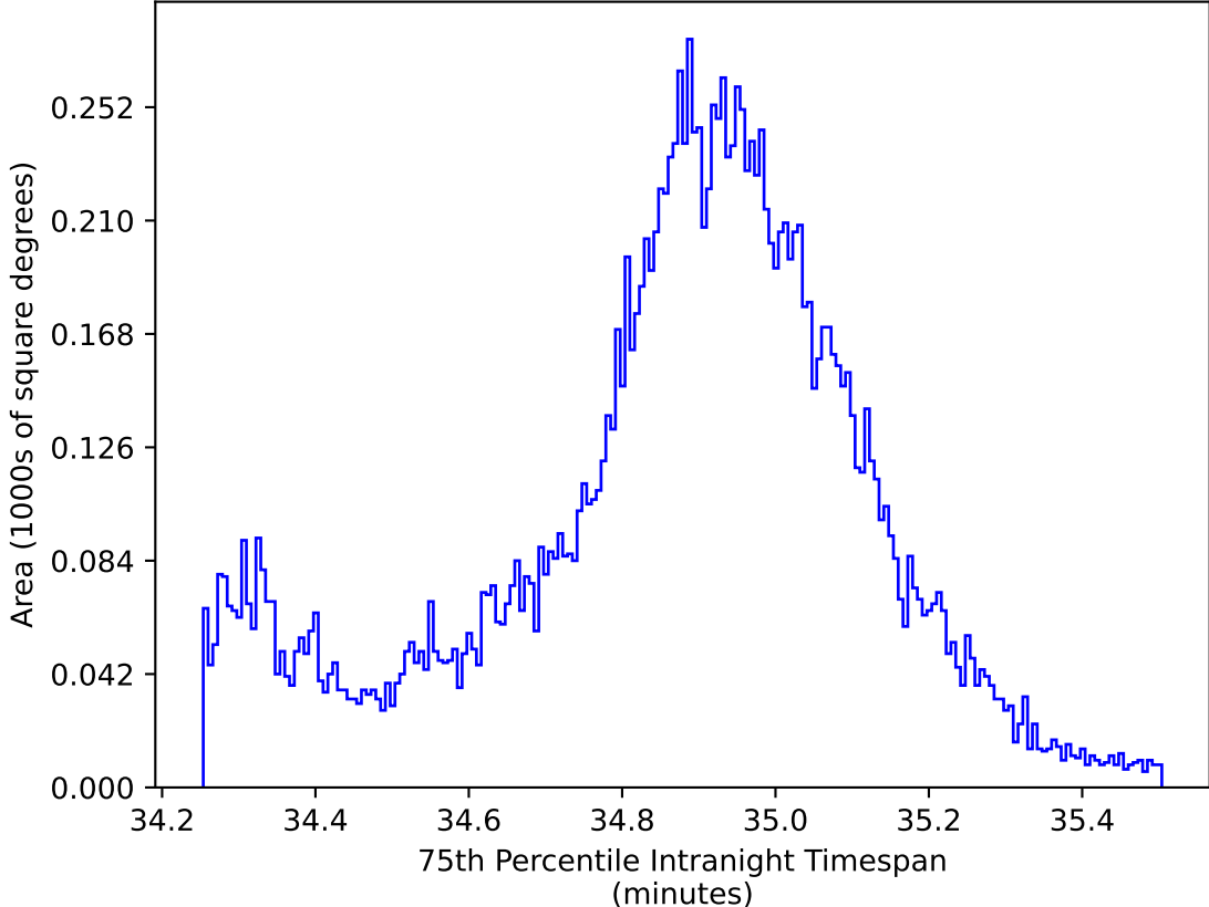
too_elab_heavy_r32_d2_gz_v3.4_10yrs WFD all bands: 75th Percentile Intranight Timespan
