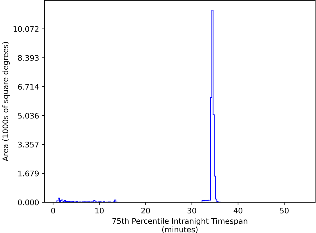
too_elab_heavy_r32_d2_gz_v3.4_10yrs All sky zy bands: 75th Percentile Intranight Timespan
