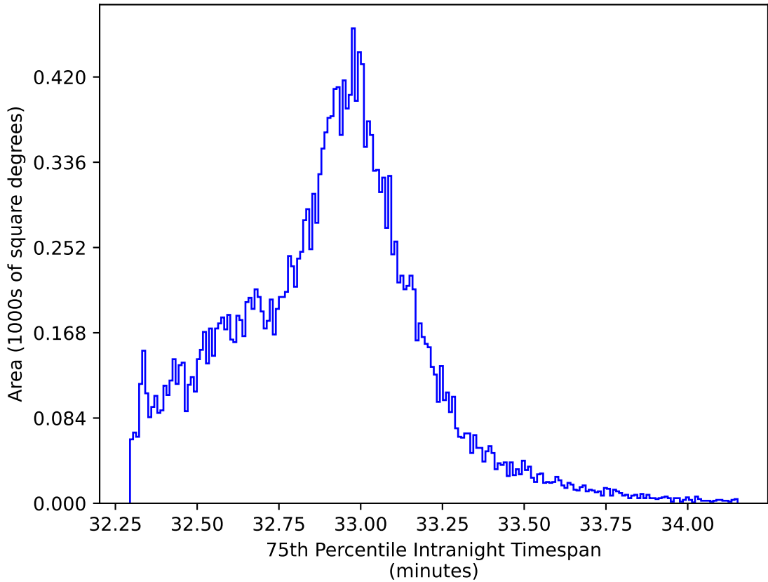
too_elab_heavy_r32_d2_gz_v3.4_10yrs All sky y band: 75th Percentile Intranight Timespan
