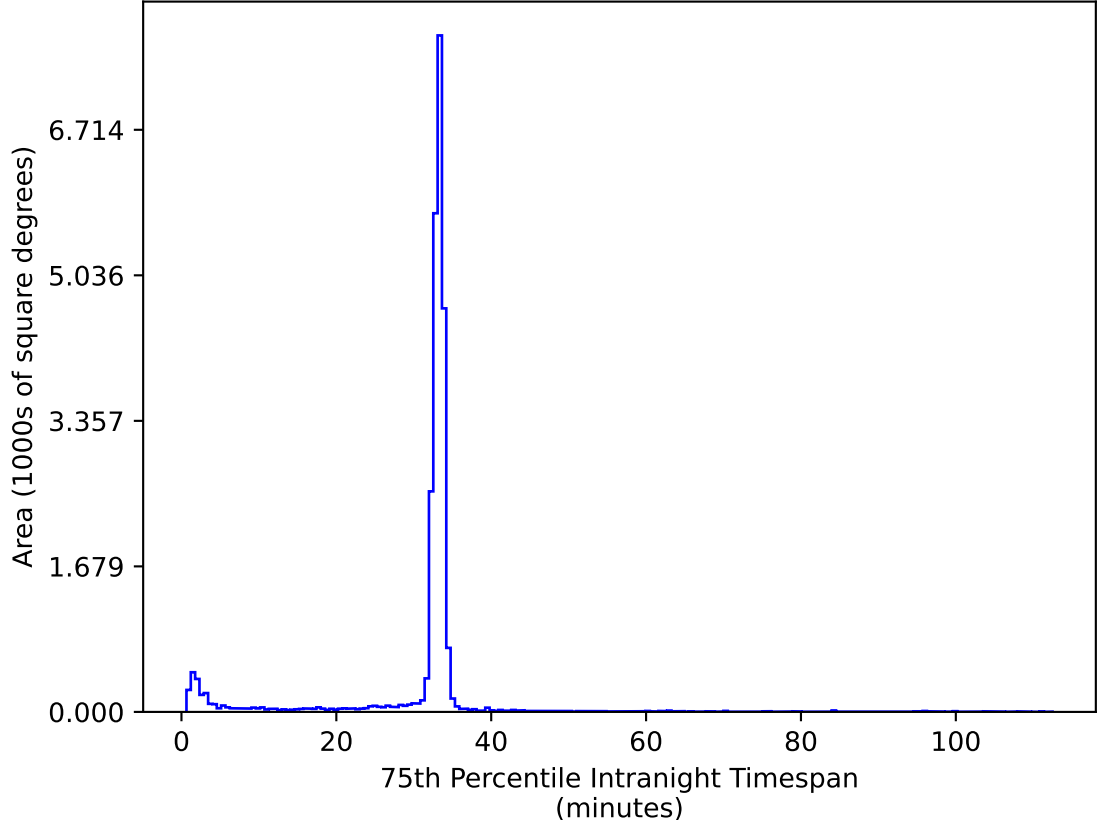
too_elab_heavy_r32_d2_gz_v3.4_10yrs All sky ug bands: 75th Percentile Intranight Timespan
