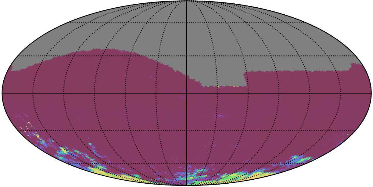
too_elab_heavy_r32_d2_gz_v3.4_10yrs All sky ri bands: 75th Percentile Intranight Timespan
