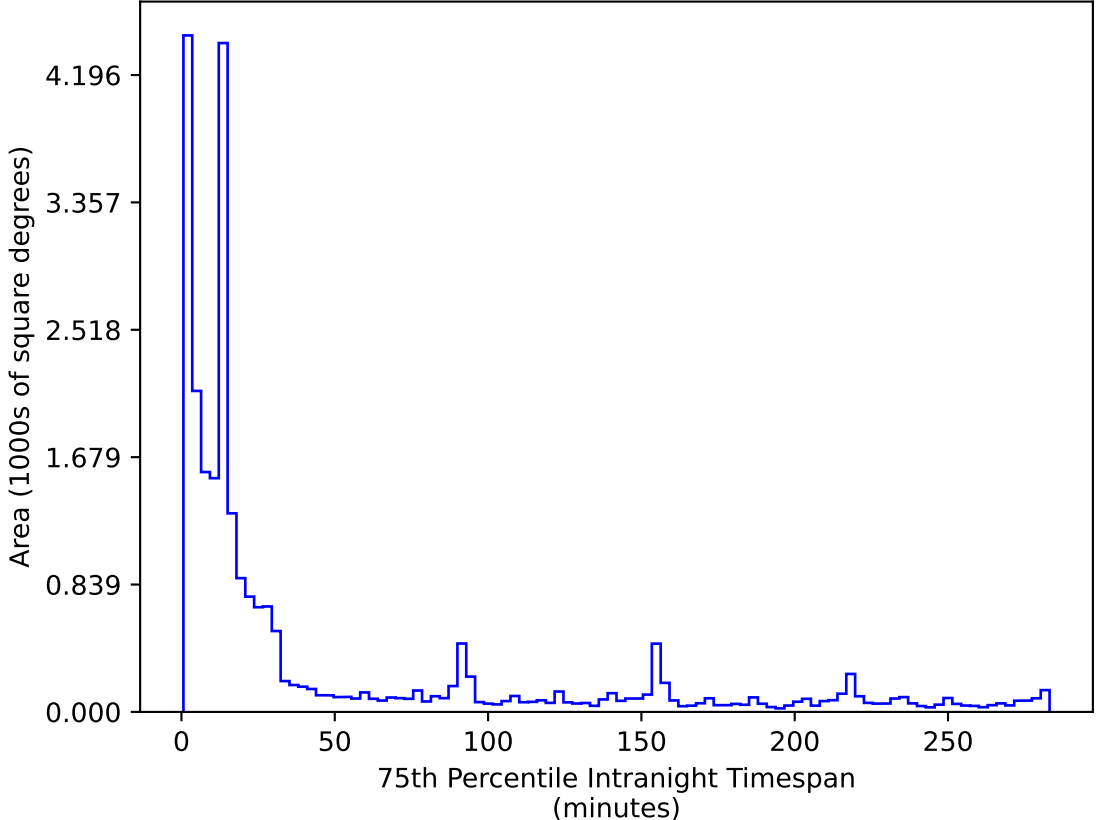
too_elab_heavy_r32_d2_gz_v3.4_10yrs All sky r band: 75th Percentile Intranight Timespan
