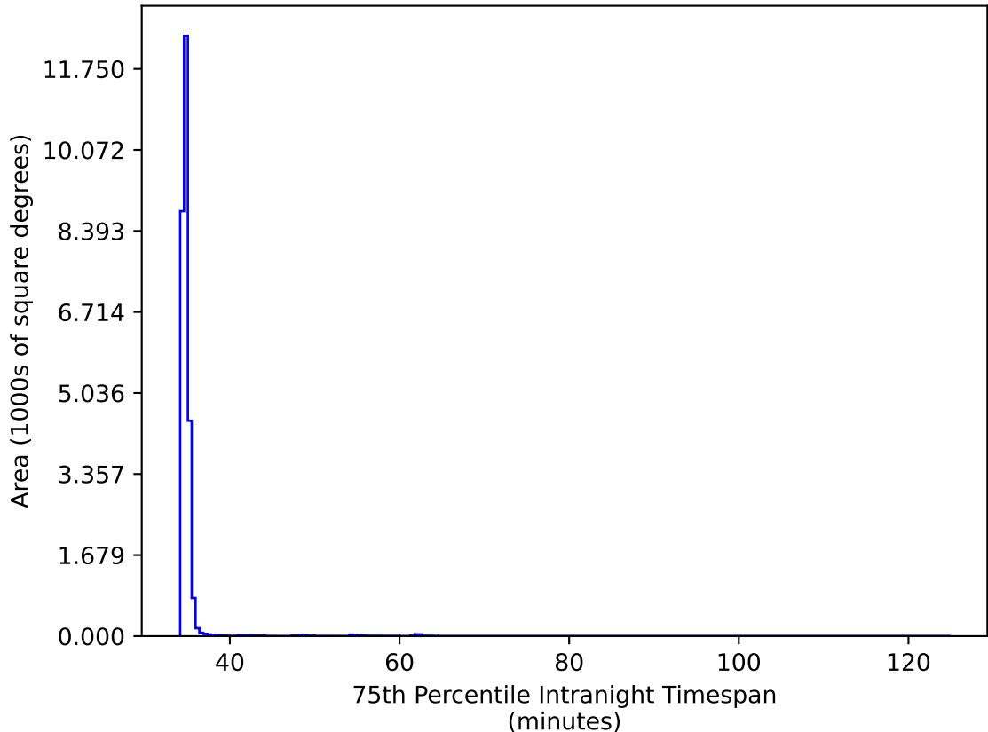
too_elab_heavy_r32_d2_gz_v3.4_10yrs All sky iz bands: 75th Percentile Intranight Timespan
