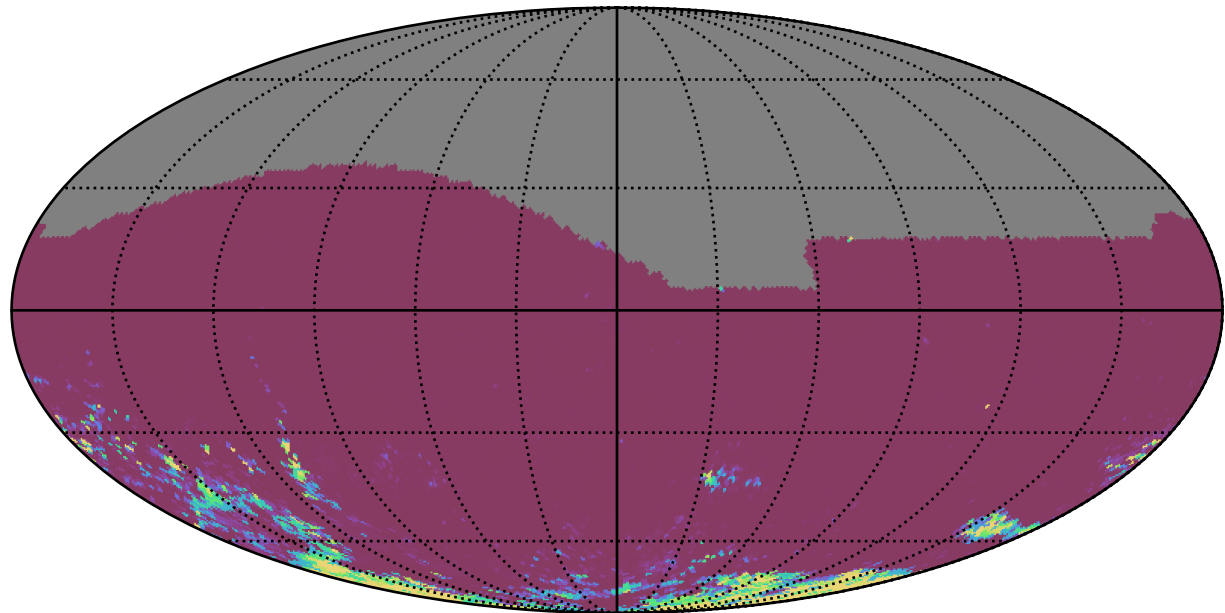
too_elab_heavy_r32_d2_gz_v3.4_10yrs All sky gr bands: 75th Percentile Intranight Timespan
