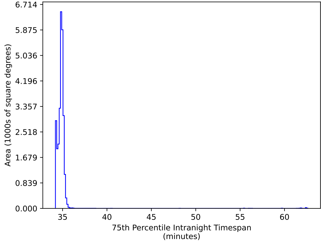
too_elab_heavy_r32_d2_gz_v3.4_10yrs All sky: 75th Percentile Intranight Timespan
