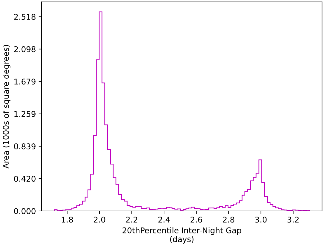
too_elab_heavy_r32_d2_gz_v3.4_10yrs WFD z band: 20thPercentile Inter-Night Gap
