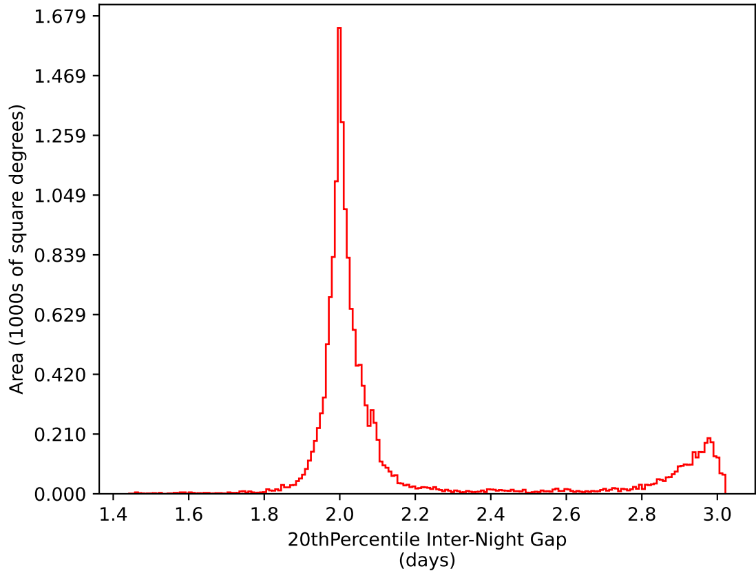
too_elab_heavy_r32_d2_gz_v3.4_10yrs WFD i band: 20thPercentile Inter-Night Gap
