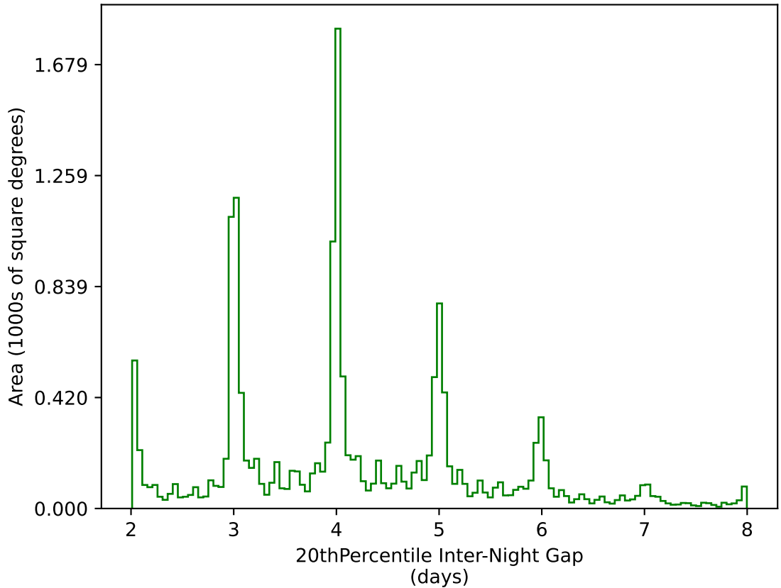
too_elab_heavy_r32_d2_gz_v3.4_10yrs WFD g band: 20thPercentile Inter-Night Gap
