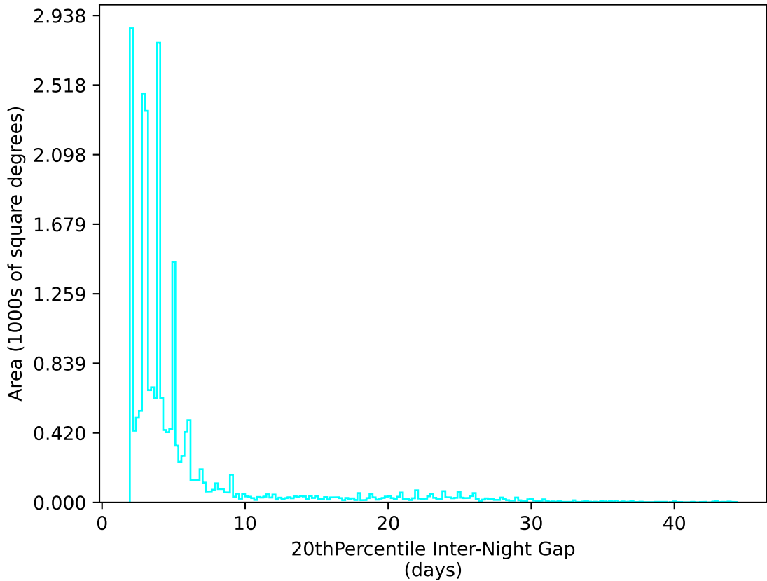
too_elab_heavy_r32_d2_gz_v3.4_10yrs All sky u band: 20thPercentile Inter-Night Gap
