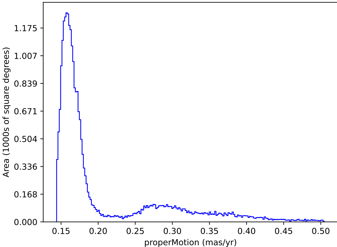
too_elab_heavy_r32_d2_gz_v3.4_10yrs : properMotion
