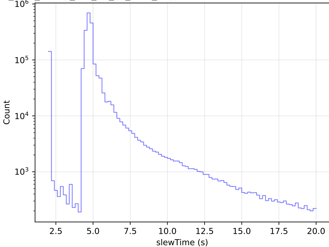
too_elab_heavy_r32_d2_gz_v3.4_10yrs All visits: Zoom Slew Time Histogram
