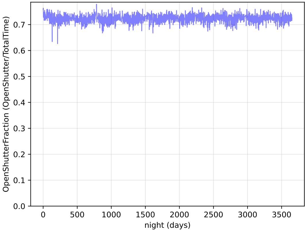
too_elab_heavy_r32_d2_gz_v3.4_10yrs : OpenShutterFraction
