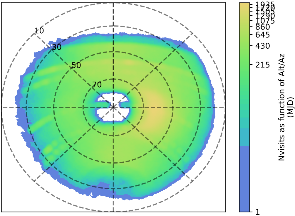
too_elab_heavy_r32_d2_gz_v3.4_10yrs y: Nvisits as function of Alt/Az
