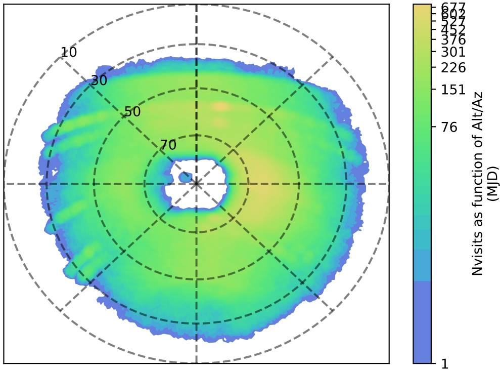
too_elab_heavy_r32_d2_gz_v3.4_10yrs u: Nvisits as function of Alt/Az
