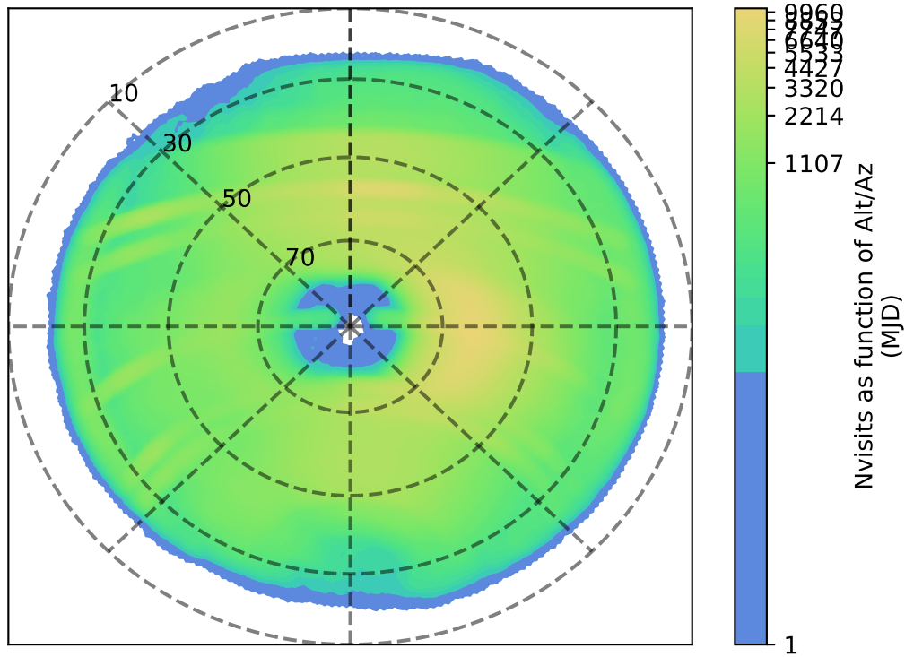
too_elab_heavy_r32_d2_gz_v3.4_10yrs : Nvisits as function of Alt/Az
