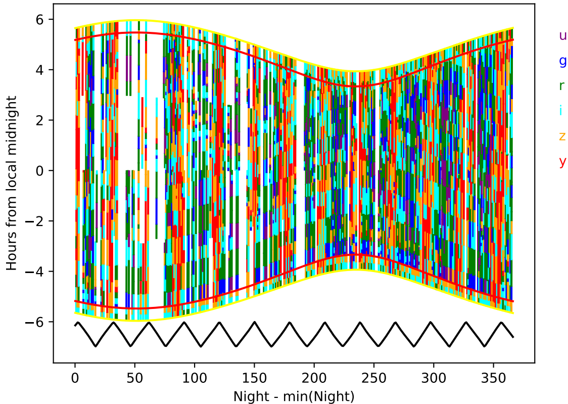
too_elab_heavy_r32_d2_gz_v3.4_10yrs year 9-10: Hourglass
