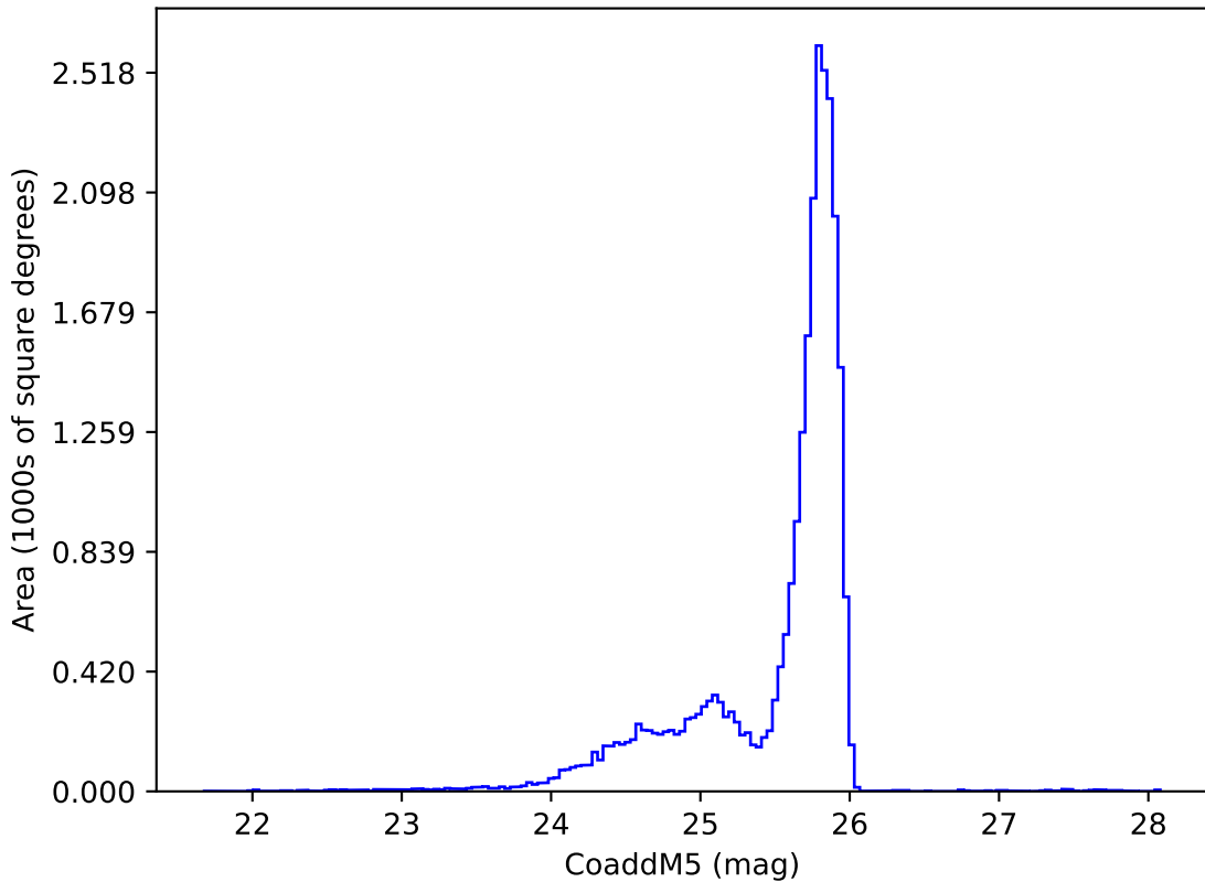
too_elab_heavy_r32_d2_gz_v3.4_10yrs z: CoaddM5
