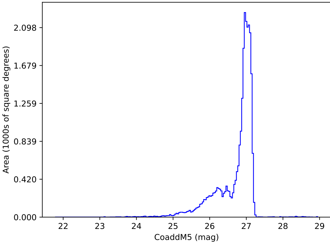
too_elab_heavy_r32_d2_gz_v3.4_10yrs r: CoaddM5
