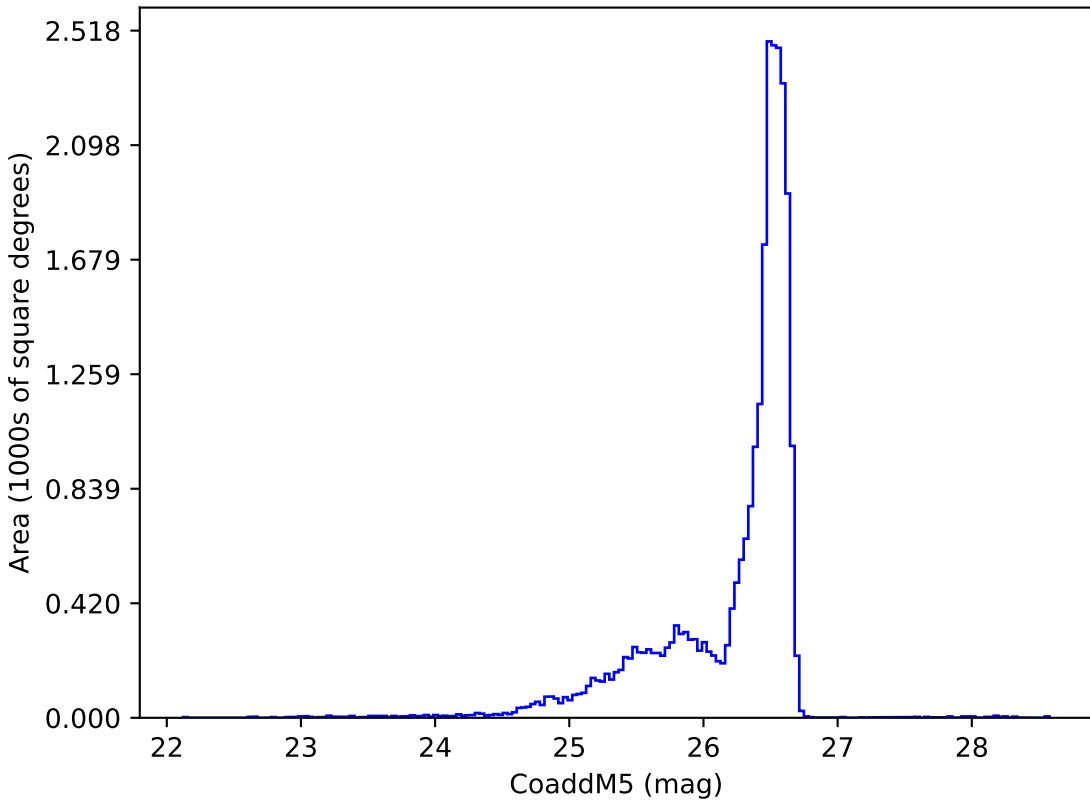
too_elab_heavy_r32_d2_gz_v3.4_10yrs i: CoaddM5
