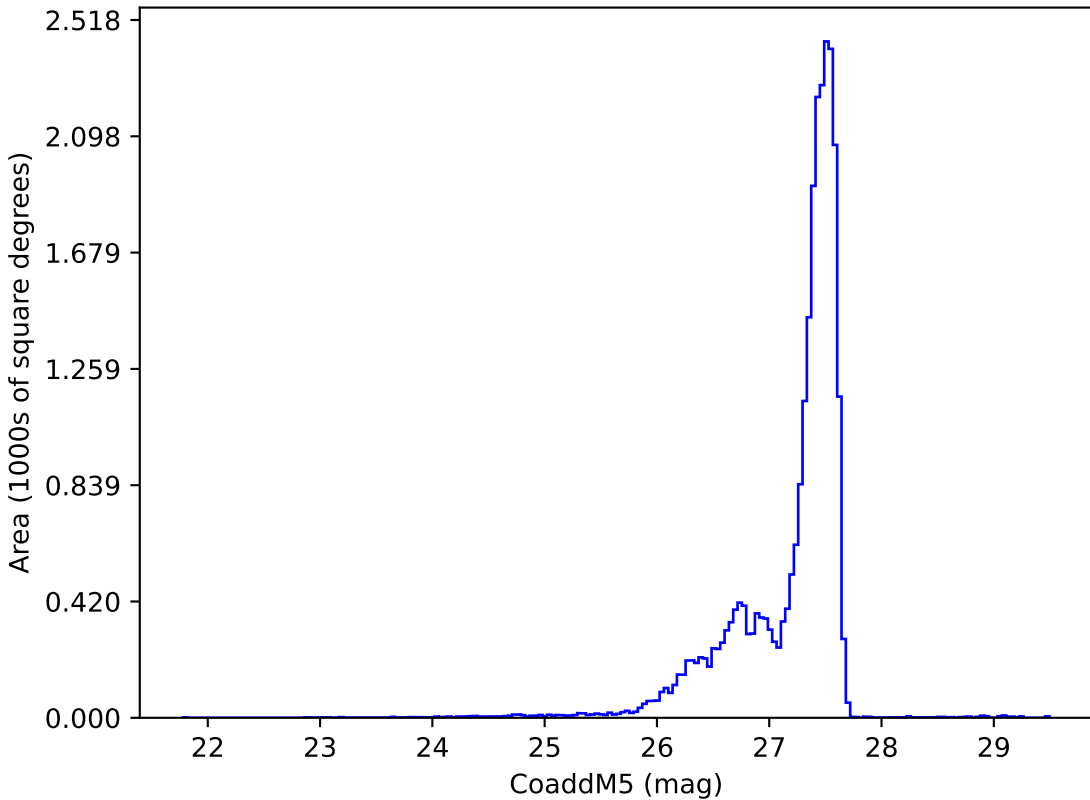
too_elab_heavy_r32_d2_gz_v3.4_10yrs : CoaddM5
