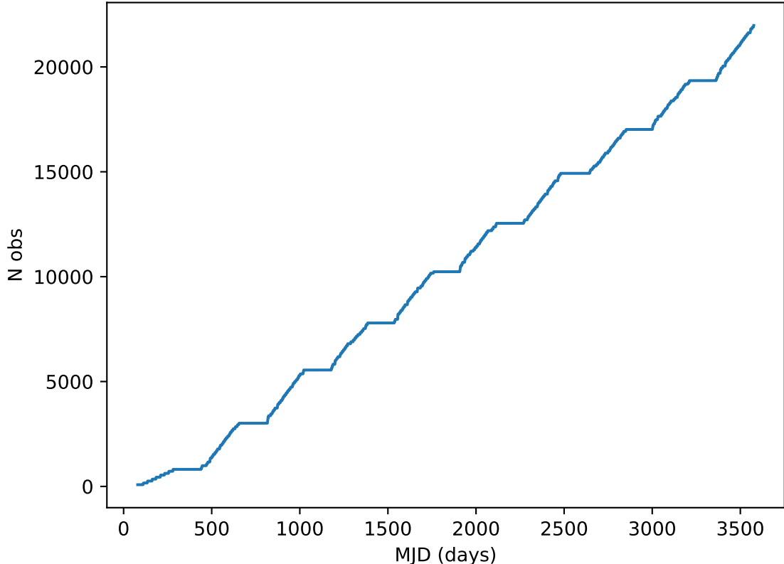
too_elab_heavy_r32_d2_gz_v3.4_10yrs all bands: DD:XMM_LSS Cumulative NVisits
