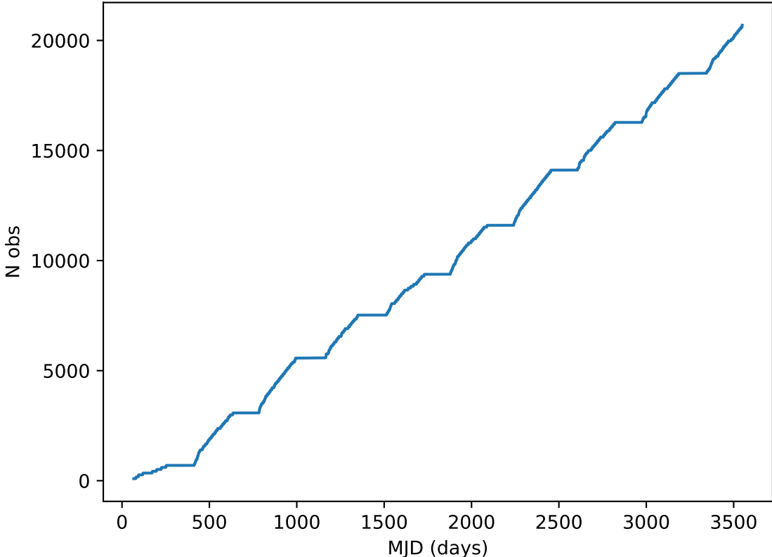
too_elab_heavy_r32_d2_gz_v3.4_10yrs all bands: DD:ELAISS1 Cumulative NVisits
