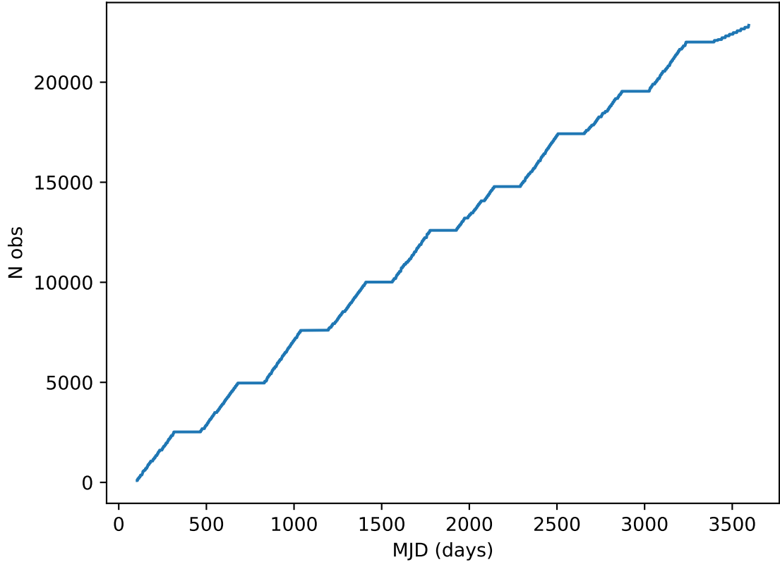
too_elab_heavy_r32_d2_gz_v3.4_10yrs all bands: DD:EDFS Cumulative NVisits
